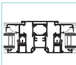
Mullion vent/vent
