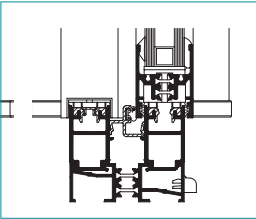
HSW sill
