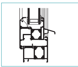
Cill/vent
