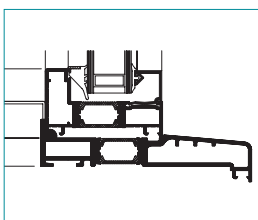
Cill/fix light
